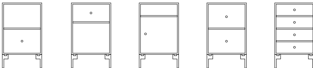
Bedside tables on legs W 35.4 cm H 46.8 cm Legs 12.6 cm
