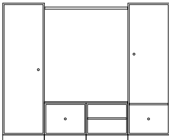
W 190.4 cm H 150.2/36.2 cm Plinth 7 cm
